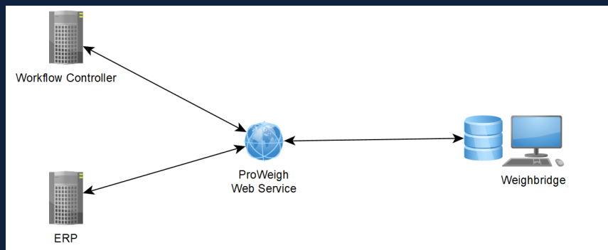
Figure 1: Webservices
